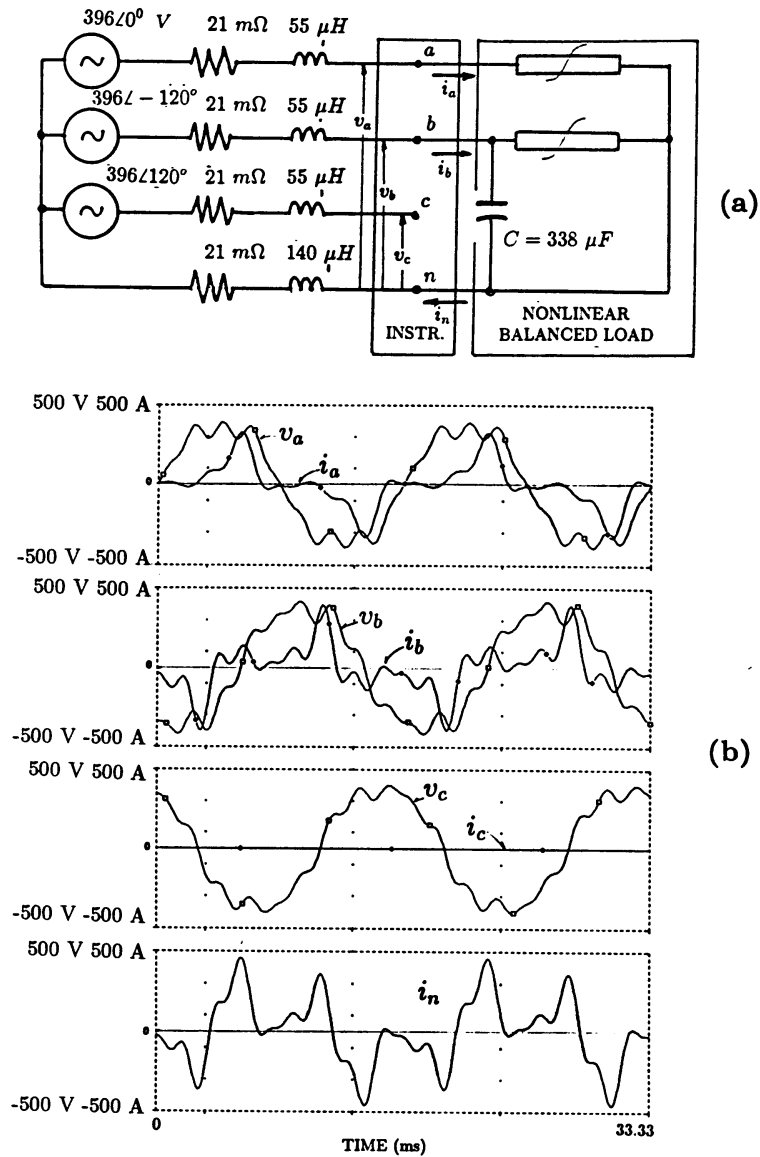
Figure A.3—Three-Phase, four-wire circuit with a nonlinear unbalanced load
